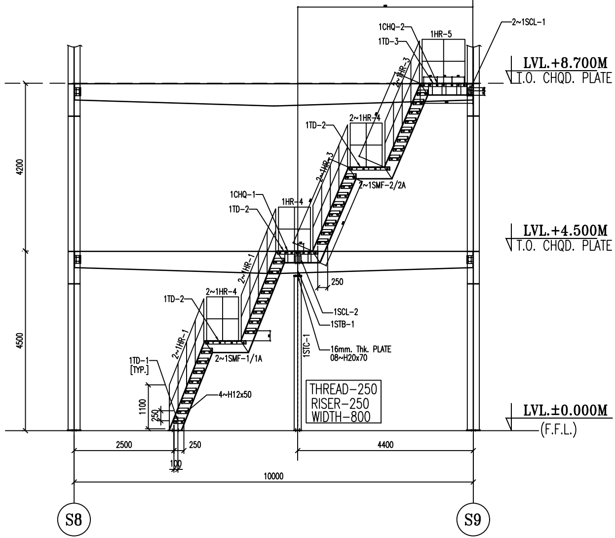
DETAIL OF STAIR CASE-1&3
